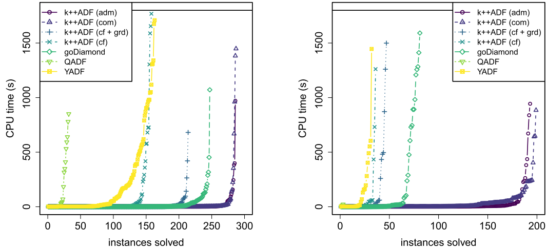
Fig. 13. Solver comparison for Skept prf : number of solved instances (on the x-axis) given a per-instance time limit (on the y-axis) for ICCMA'17 (ABA2AF, Planning, Traffic; left) and ICCMA'19 (right) instances.
