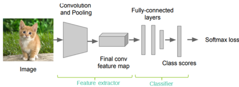
Figure 1.9: General CNN architecture, composed of a feature extractor and a classifier.
