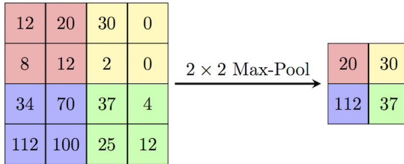
Figure 1.8: The result of a max pool operation using 2x2 blocks.
