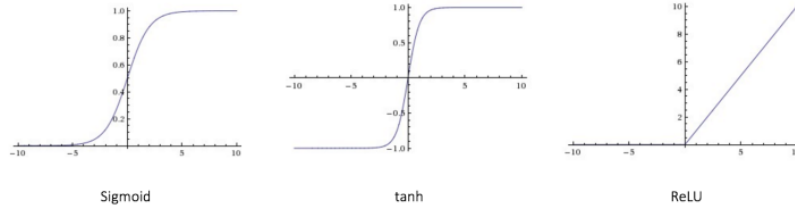
Figure 1.2: Some of the most used activation functions.
