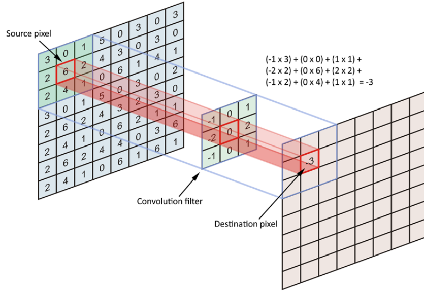
Figure 1.7: The result of a single convolution operation. The process is repeated by shifting the filter all-over the entire original image.
